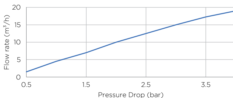
Pressure drop chart of Aquamatic 100
