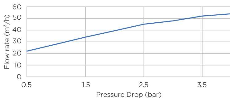
Pressure drop chart of Aquamatic 400
